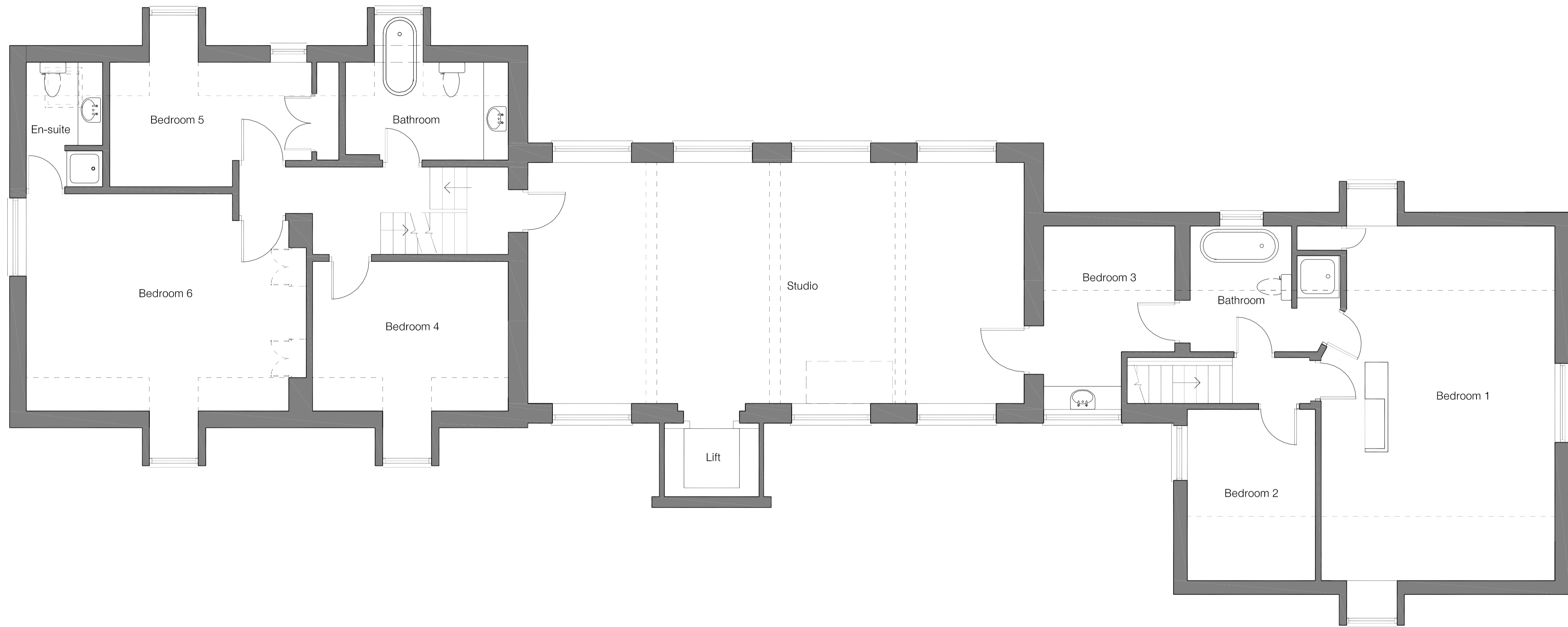
Knighton Mill 1:50 Existing First Floor Plan
