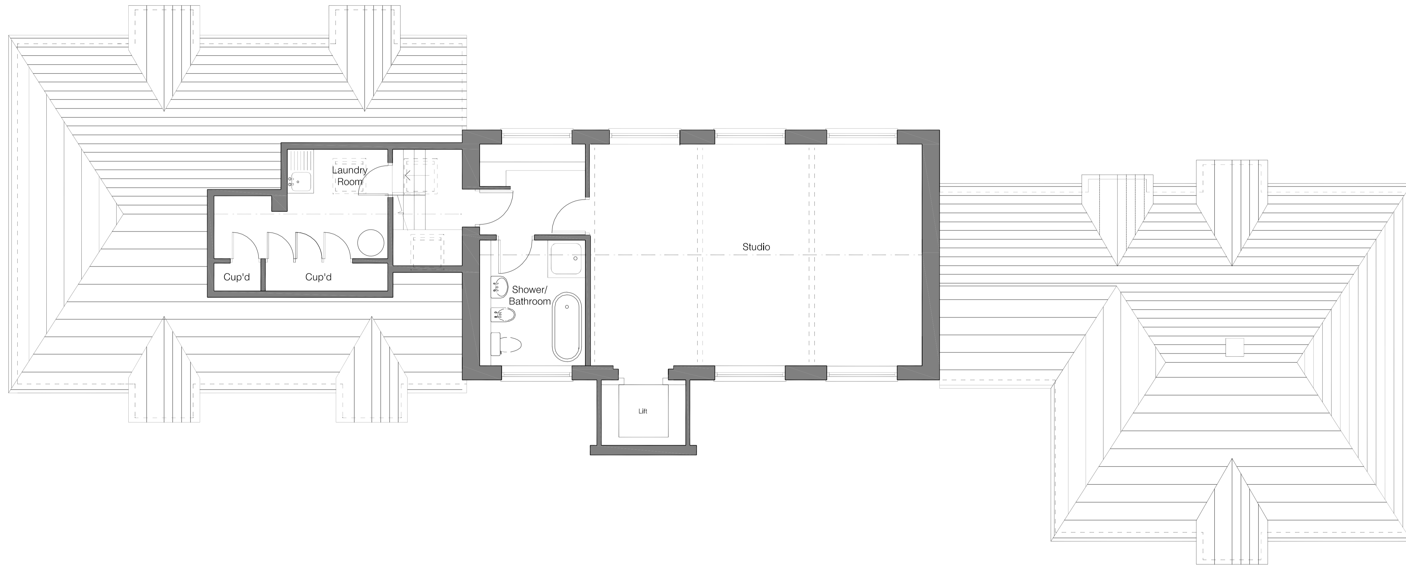
Knight Mill 1:50 Existing Second Floor Plan
