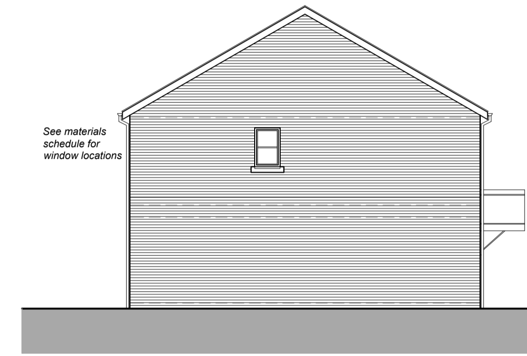
Side Elevation
