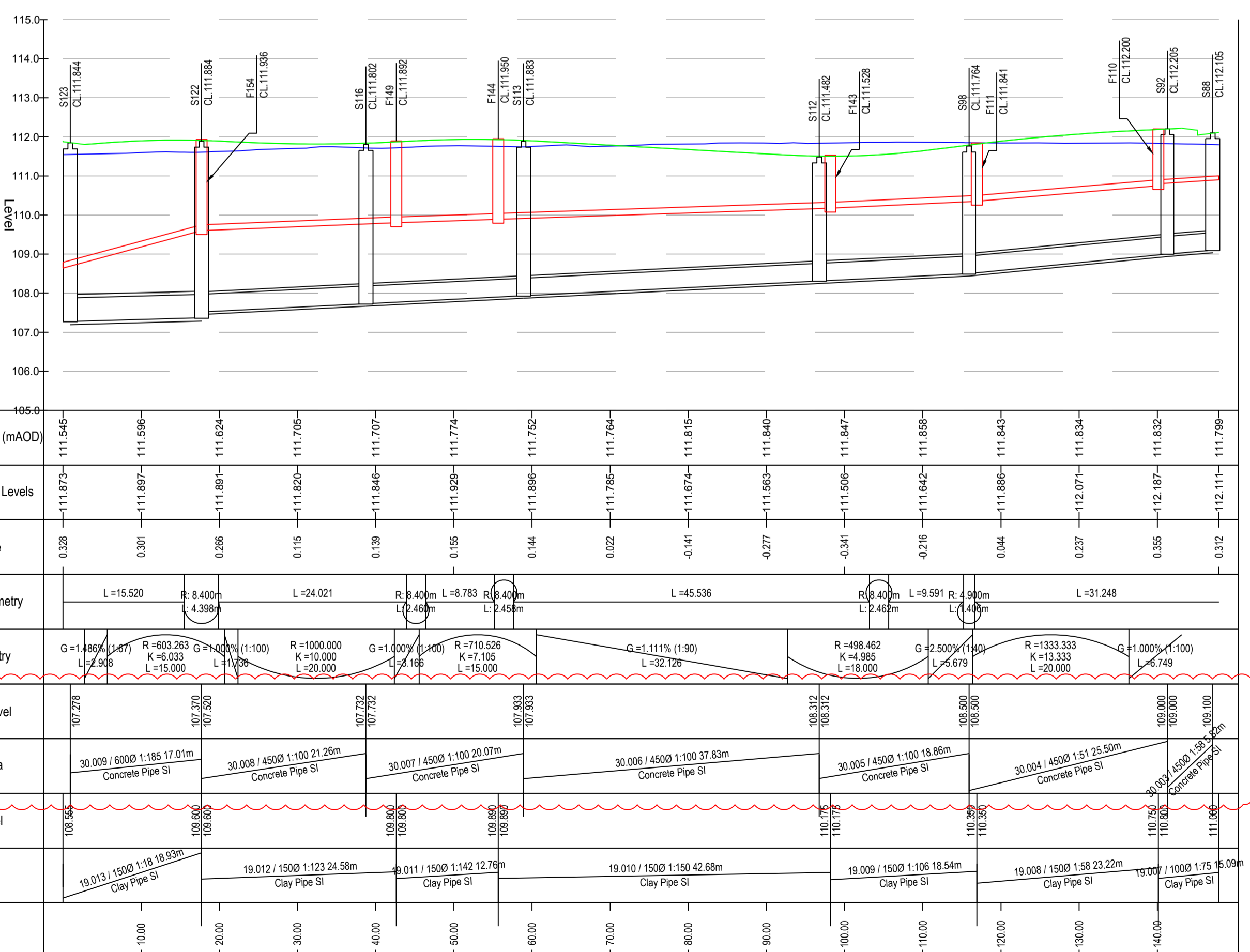
Shared Surface 18 LONG SECTION Datum: 105.00, Chainage: 0.000 - 147.884 SCALE: H 1:500, V 1:100
