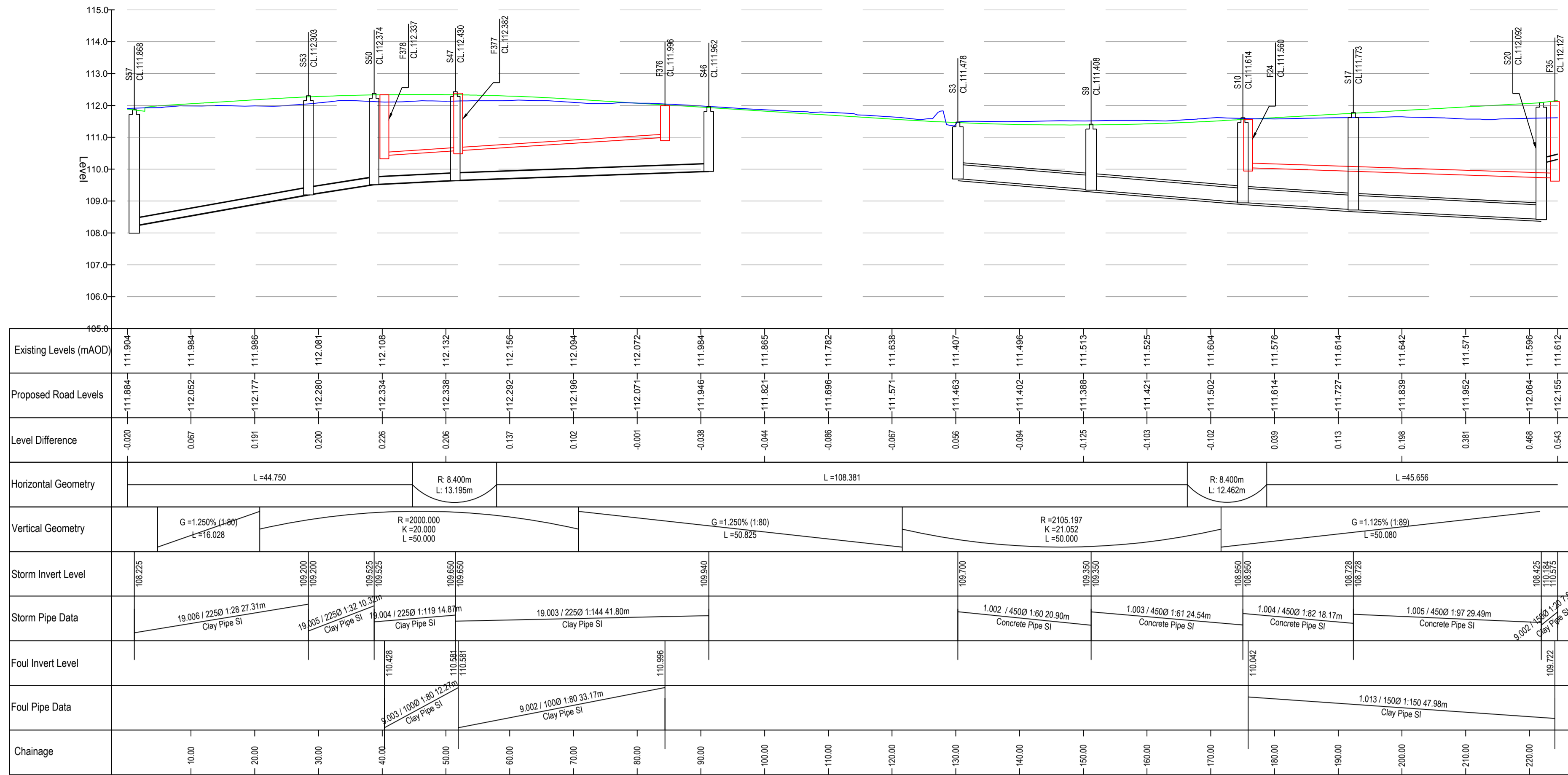
Shared Surface 17 LONG SECTION Datum: 105.00, Chainage: 0.000 - 224.443 SCALE: H 1:500, V 1:100
