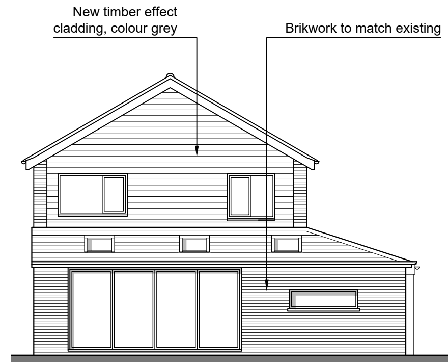
Rear Elevation
