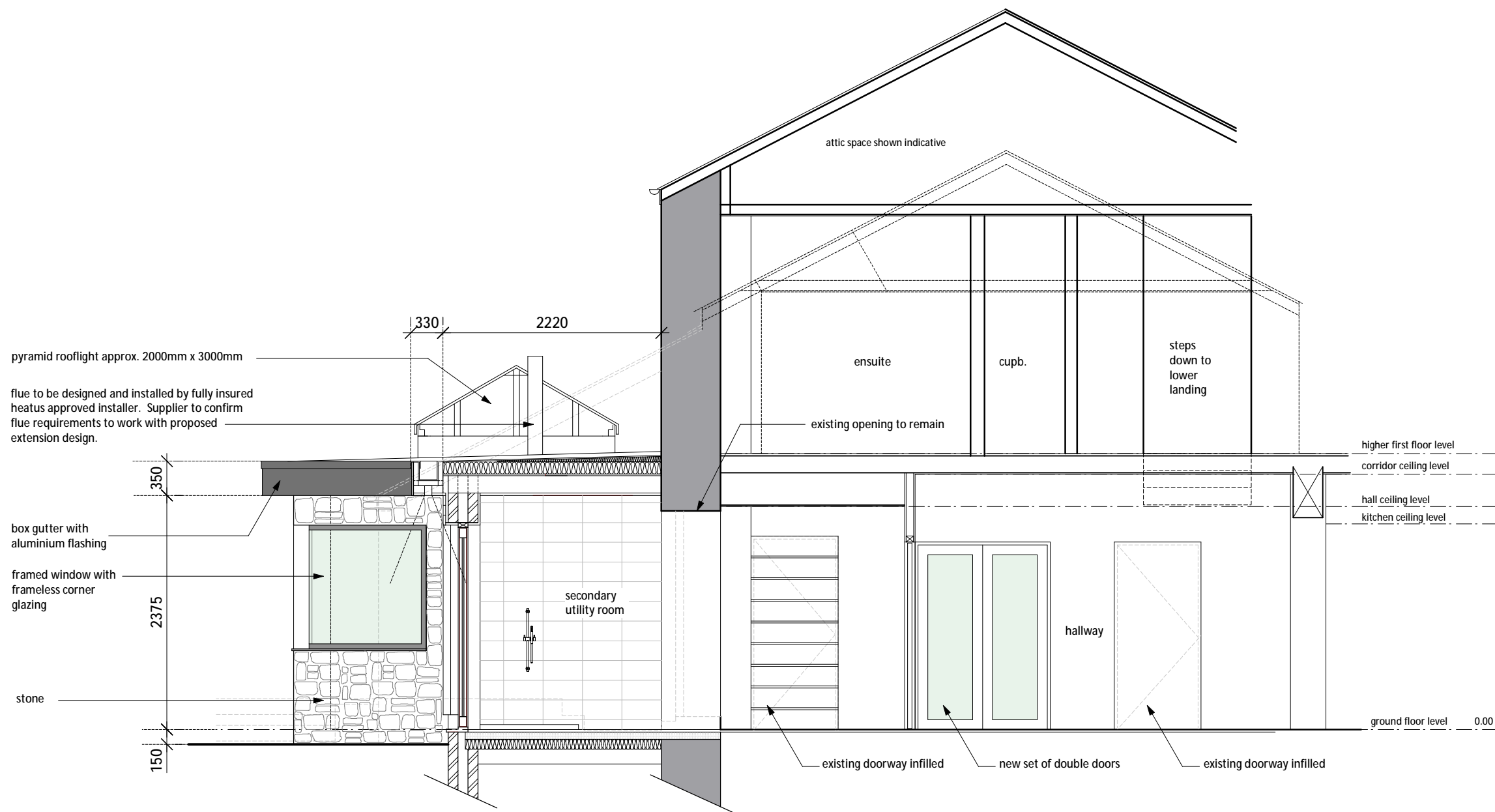
Section A:A Section through proposed secondary utility room and existing hall
