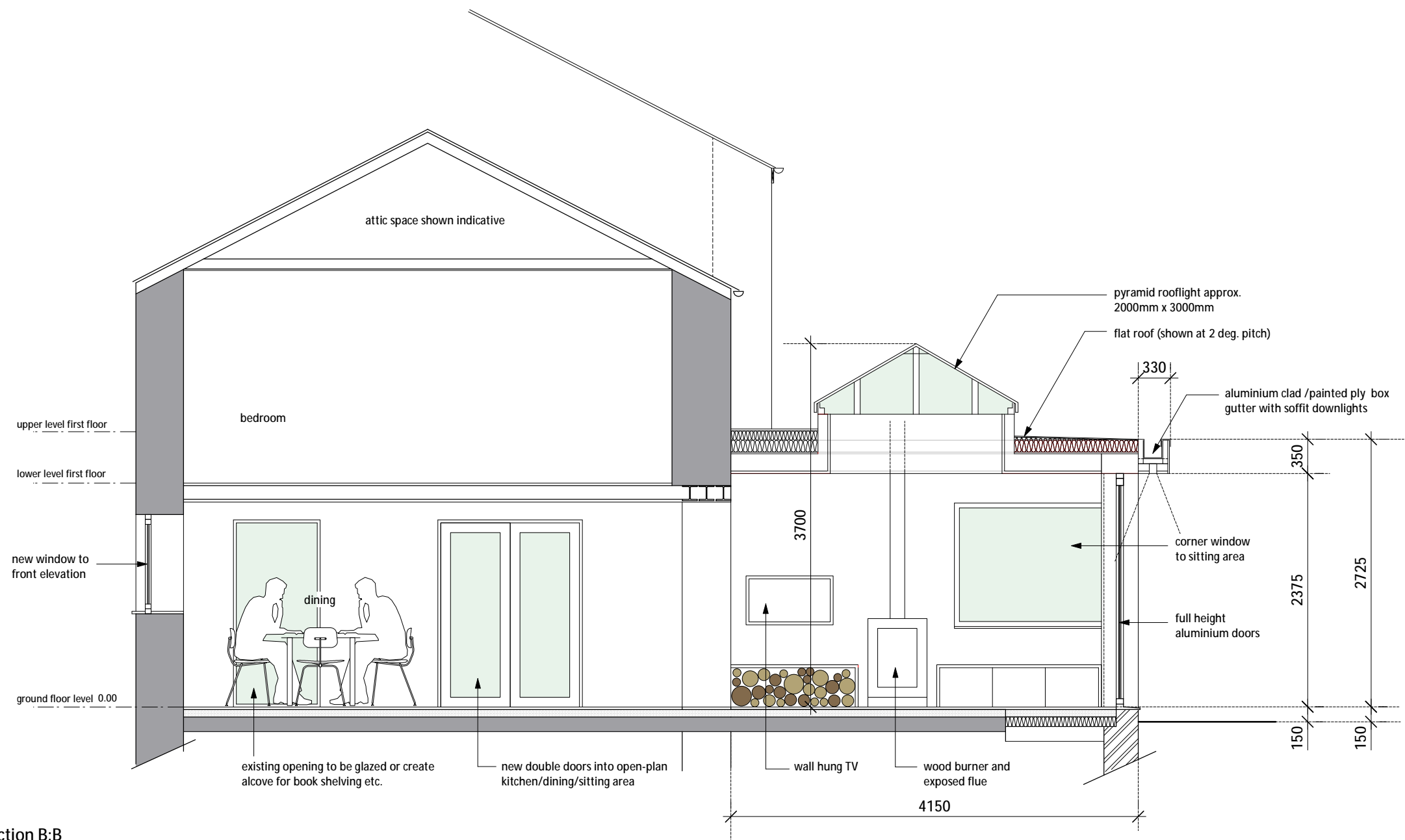
Section B:B Section through proposed dining and sitting area
